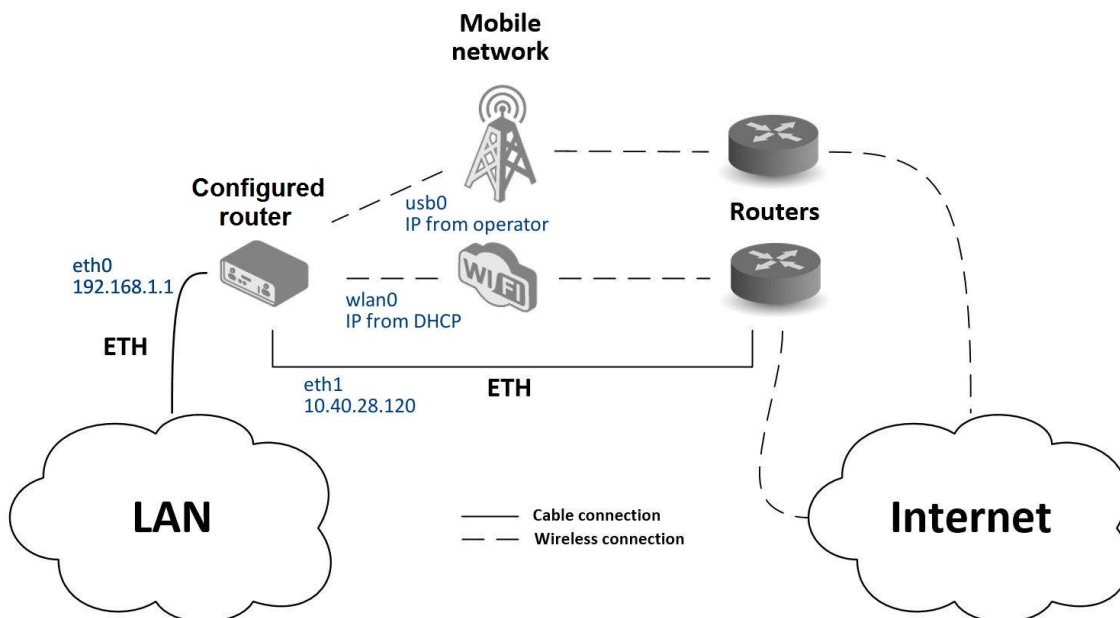
Figure 92: Backup access to the Internet – sample topology
