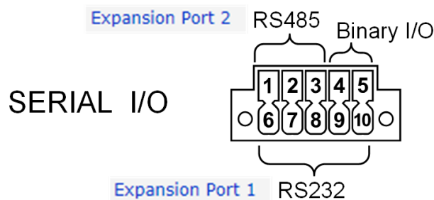
Figure 66: SERIAL I/O configuration pages overview
