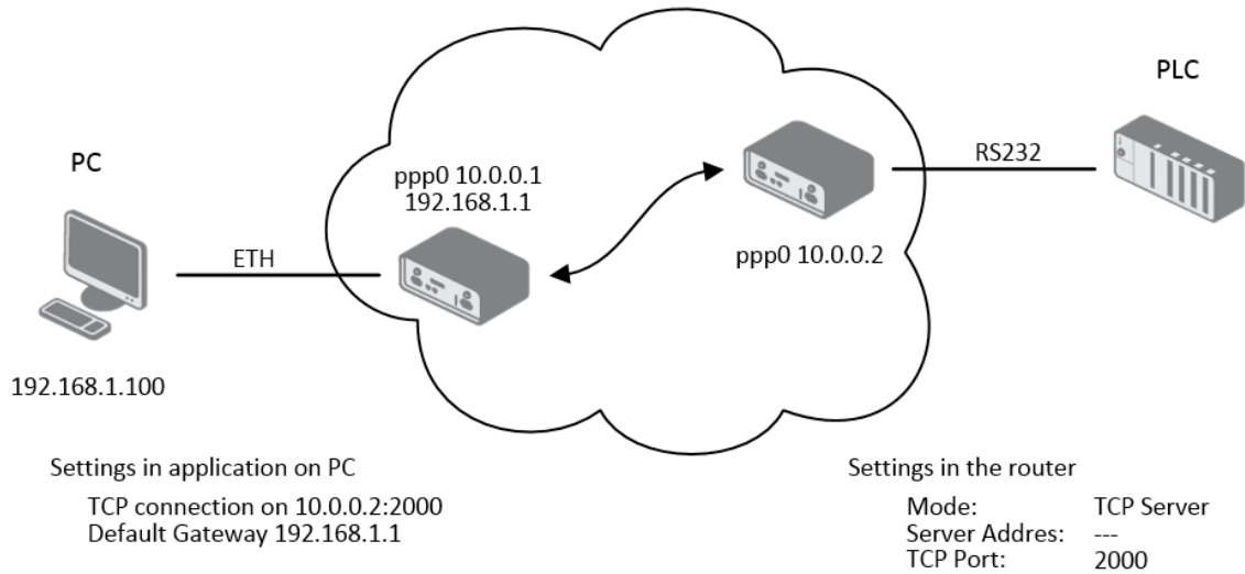
Figure 68: Example of Ethernet to serial communication configuration
