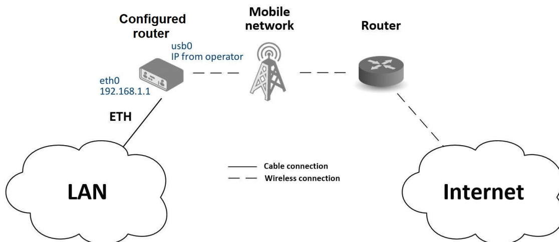
Figure 89: Access to the Internet from LAN – sample topology
