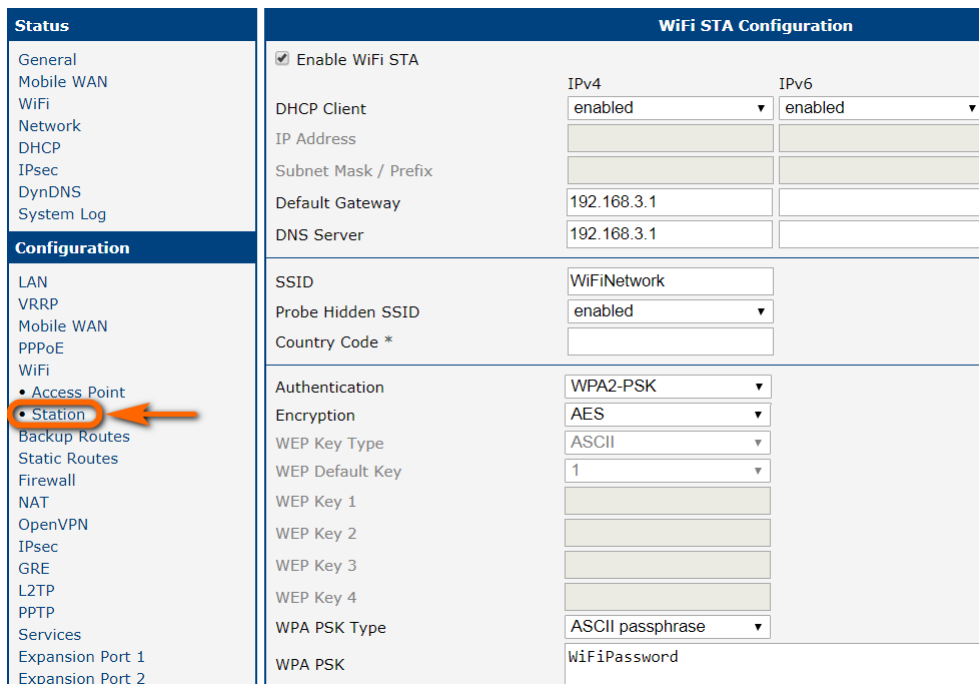
Figure 94: Backup access to the Internet – WiFi configuration
