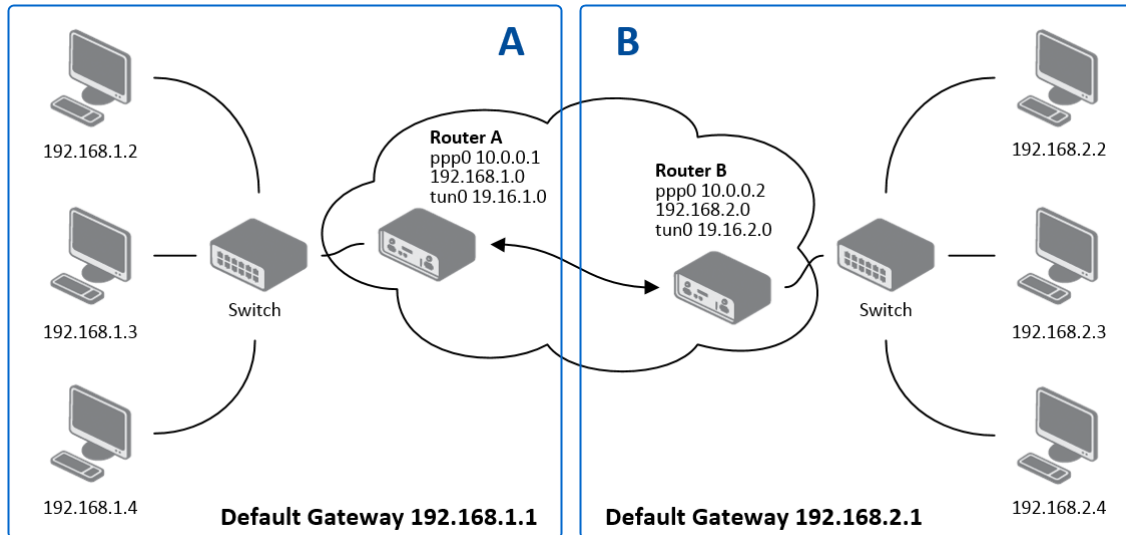
Figure 41: Topology of OpenVPN Configuration Example
