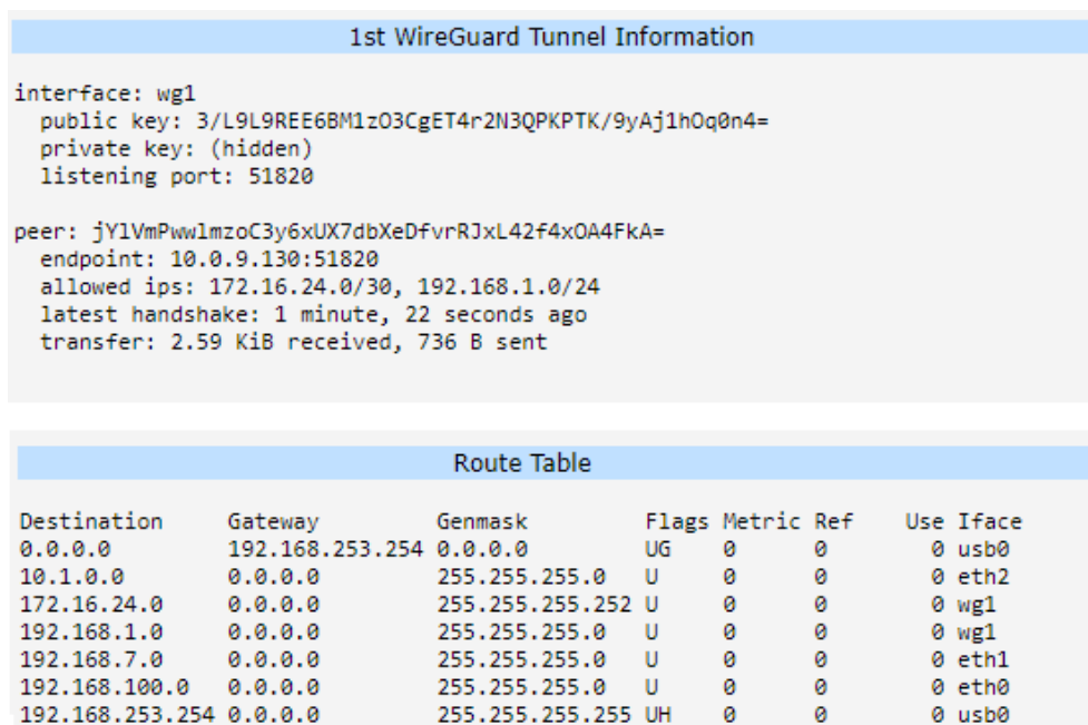
Figure 47: Router B – WireGuard Status Page and Route Table
