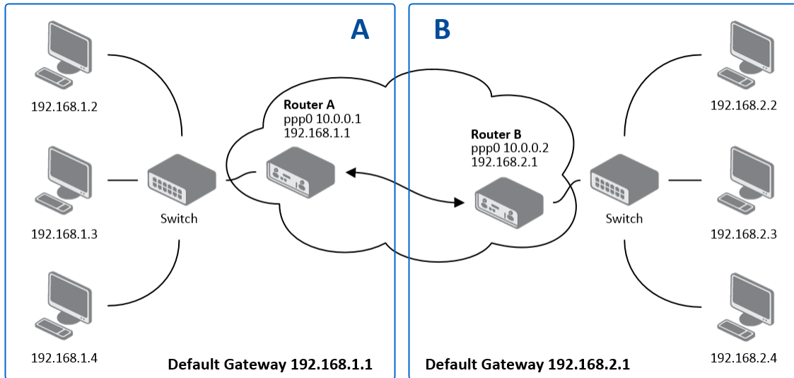
Figure 53: Topology of PPTP Tunnel Configuration Example
