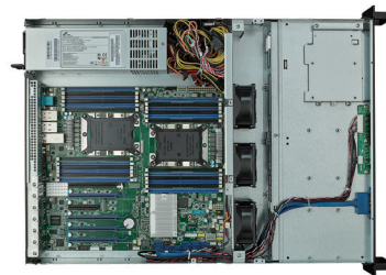
Standard 7*low-profile expansion cards version
