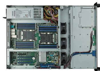
Optional 3*full-height expansion cards version
