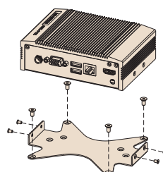
VESA mount
